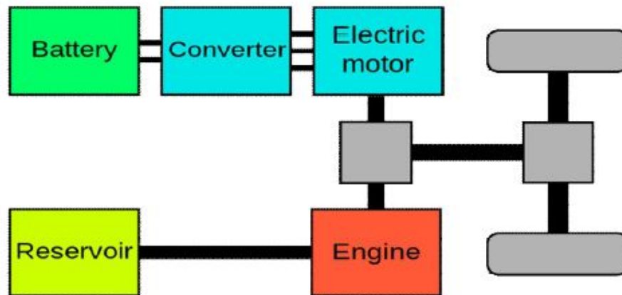
Figure 3 Parallel hybrid vehicle system
