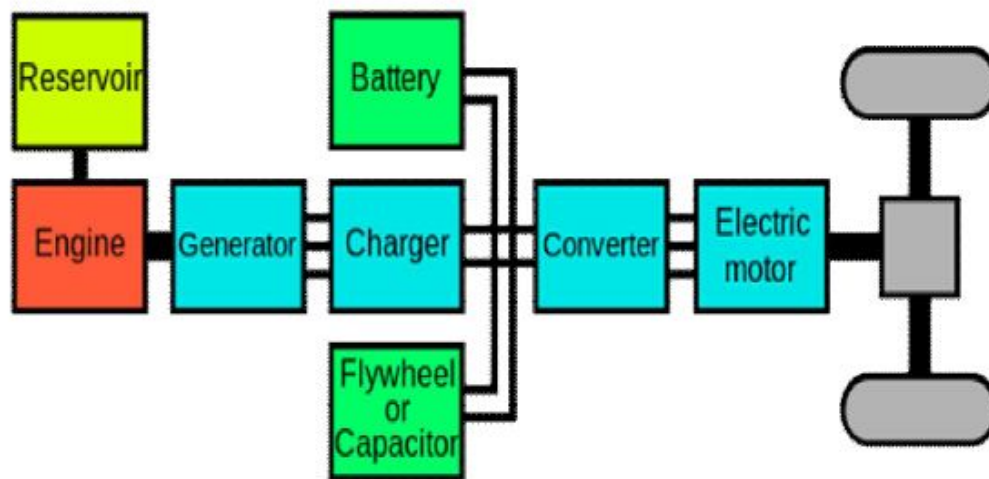
Fig. 4 HEV Series
